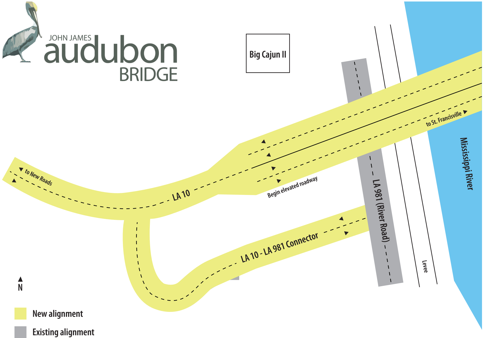
Proposed intersection of LA 981 (River Road) and new LA 10 alignment
